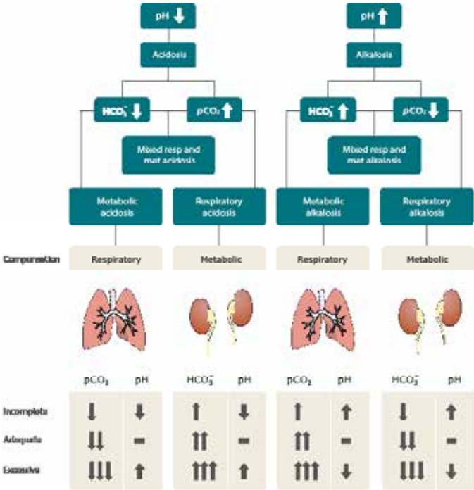
FIG. 11: Acid-base flowchart.
